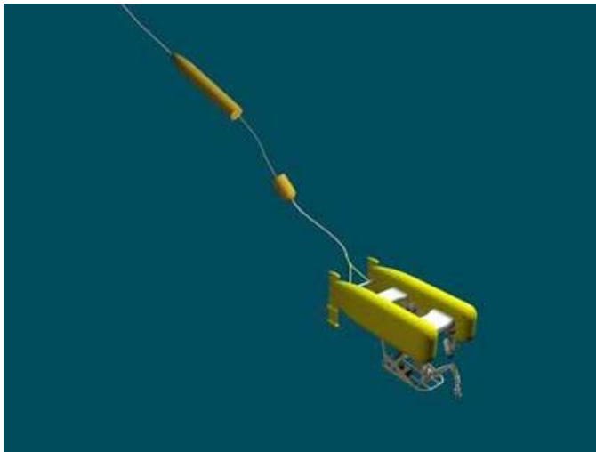
Fig. 7. Nereus showing the float-pack separating from the depressor pack.
